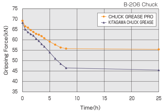
Fig.2 Grease Check Test
