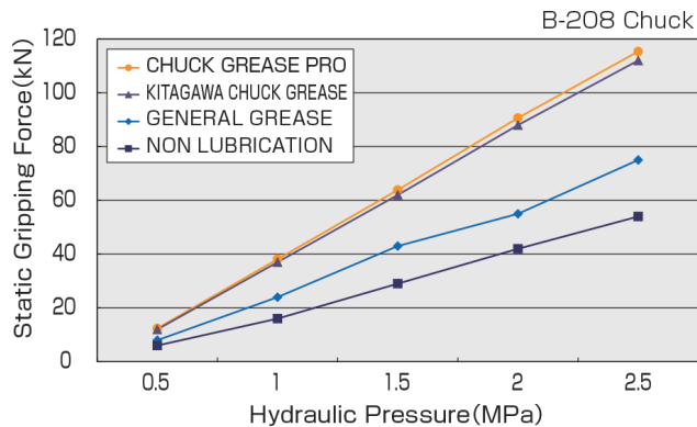
Fig.1 Gripping force check by grease
