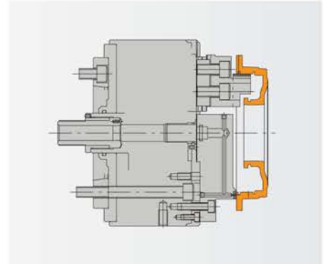
● CLUTCH
