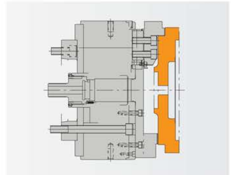
● FLYWHEEL
