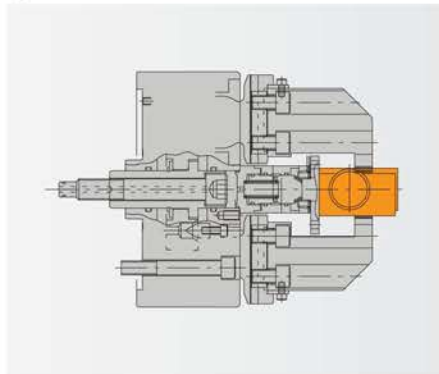
● SLEEVE
