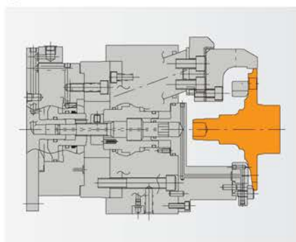
● HUB
