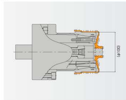
● HUB CLUTCH
