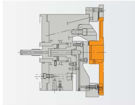
● PUMP COVER
