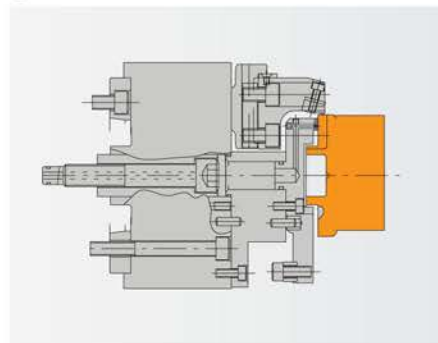
● FLYWHEEL
