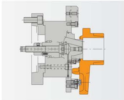
● CORE PLATE
