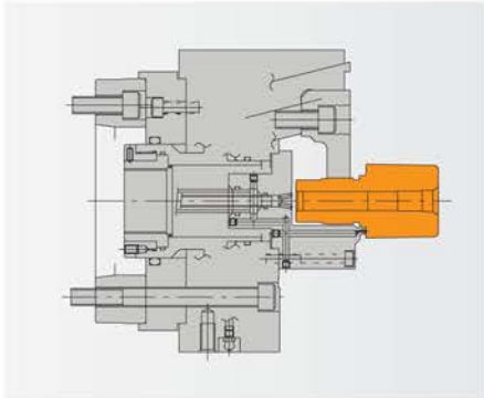
● GEAR
