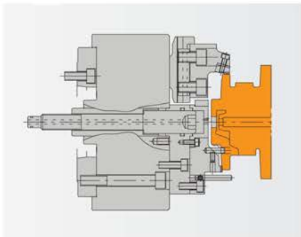
● PISTON MOTOR
