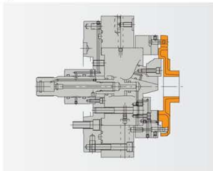
● PUMP
