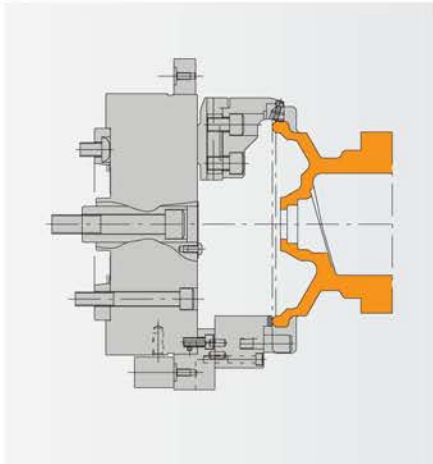
● SHAFT
