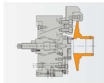
● PULLEY
