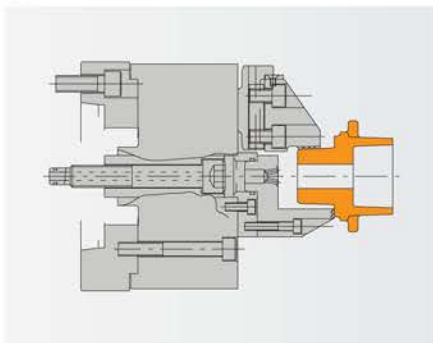
● HOUSING
