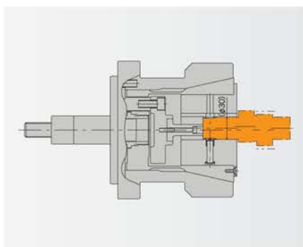
● CRANK SHAFT
