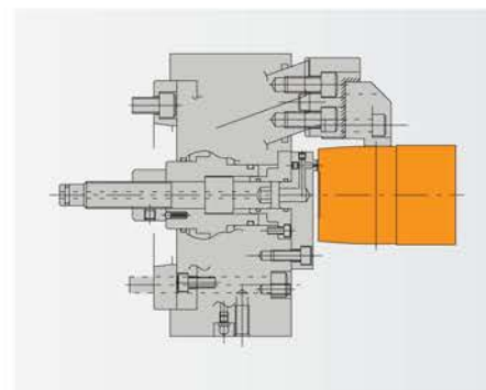
● HUB
