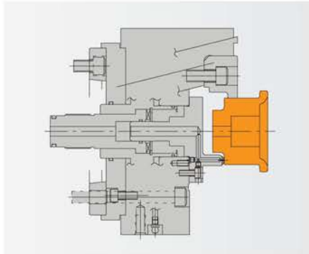
● HUB
