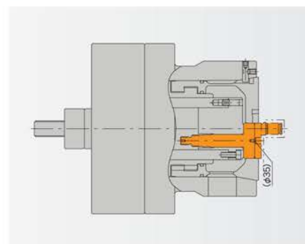
● CRANK SHAFT
