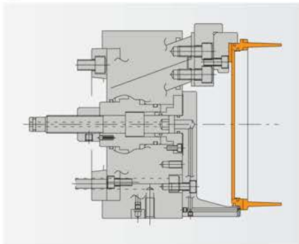
● HUB
