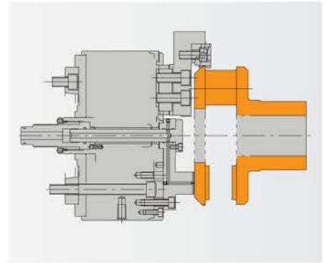
● CLUTCH
