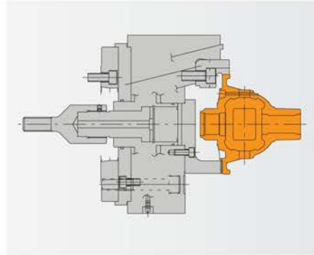
● PUMP COVER
