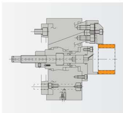
● HUB
