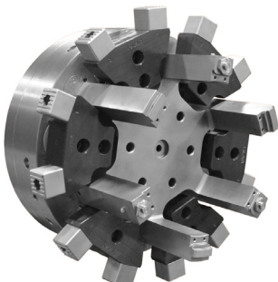
6 Jaw Ball Lock Chuck
