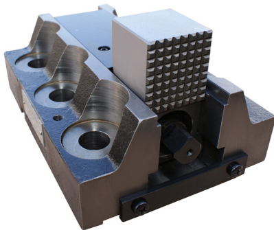
Boring Mill Jaws with 4 or More Jaw Independent Chuck Configuration
