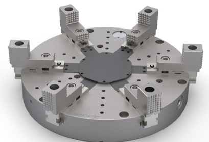
TI Low Profile, 2, 4 & 6 Jaw Manual Scroll Chucks
