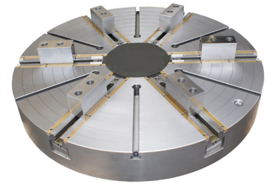
CVH 3 & 6 Self-Centering VTL Chucks
