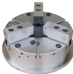
ASM 3 Jaw Stationary Chuck with Built-In Air Cylinder
