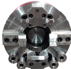
4 Jaw 2+2 Chuck
