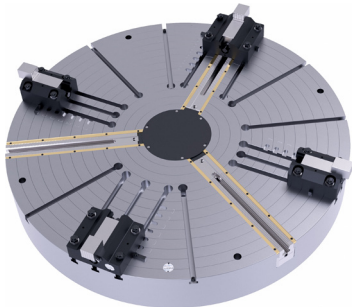
CVB Self-Centering Large VTL & Independent Combination Chucks
