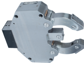
FRC Integral Steady Rests Feature an Integrated Cylinder Design
